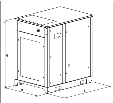
Fig. 3.2 Dimension drawing AV30-55.
